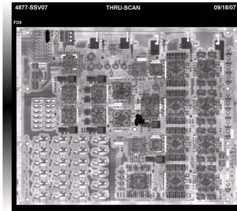
Figure 2: Through scan acoustic image of printed circuit board. The delaminations are highlighted in red
