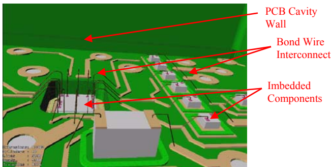
Figure 1. Active and passive components are imbedded in a cavity on a laminate substrate.
