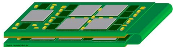
Figure 7. Bumped die, wire bonded die, and thin film passives integrated on rigid flex substrate to eliminate failure opportunities due to connector systems.
