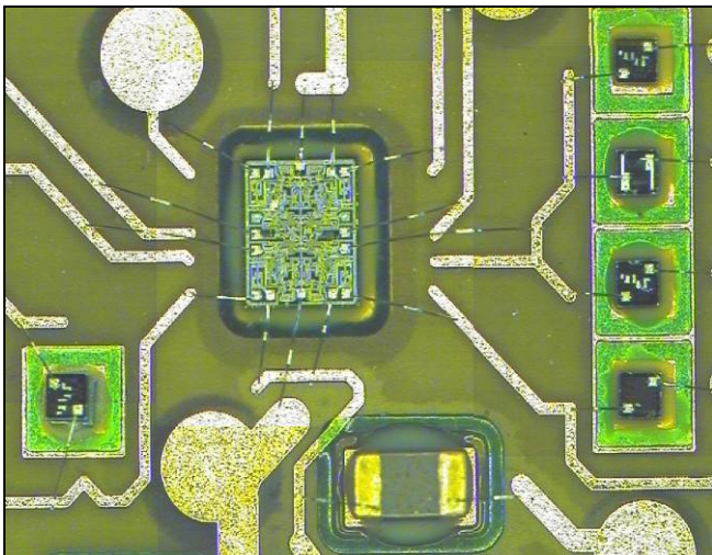
Figure 5. Wires bonded to electrically interconnect components on the prototype.
