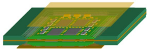
Figure 6. Bumped die, wire bonded die, and thin film passives integrated on a high density interposer imbedded within a system card.
